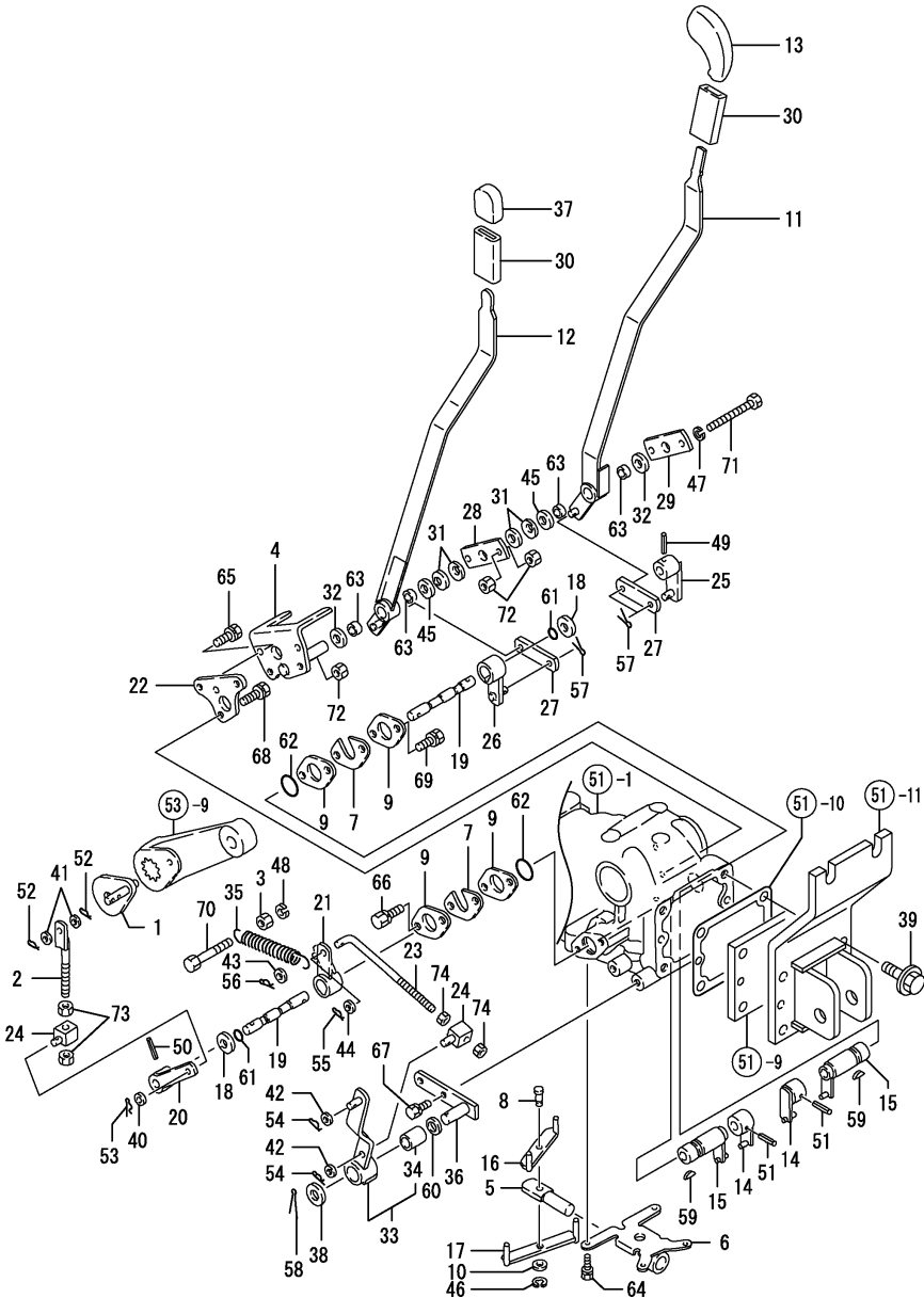
Fig.90. HYDRAULIC CONTROL(ADD.
