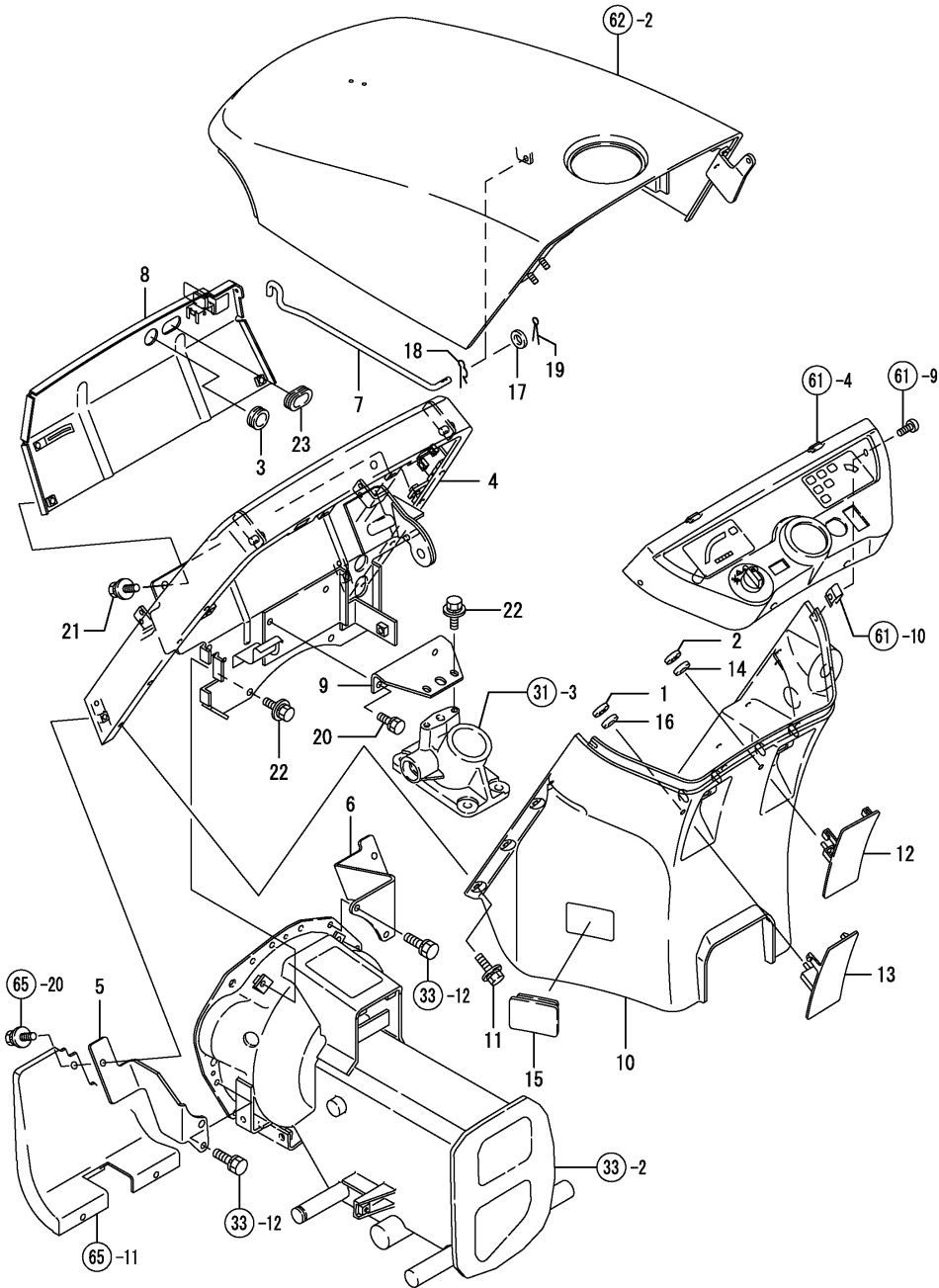
Fig.63. DASHBOARD
