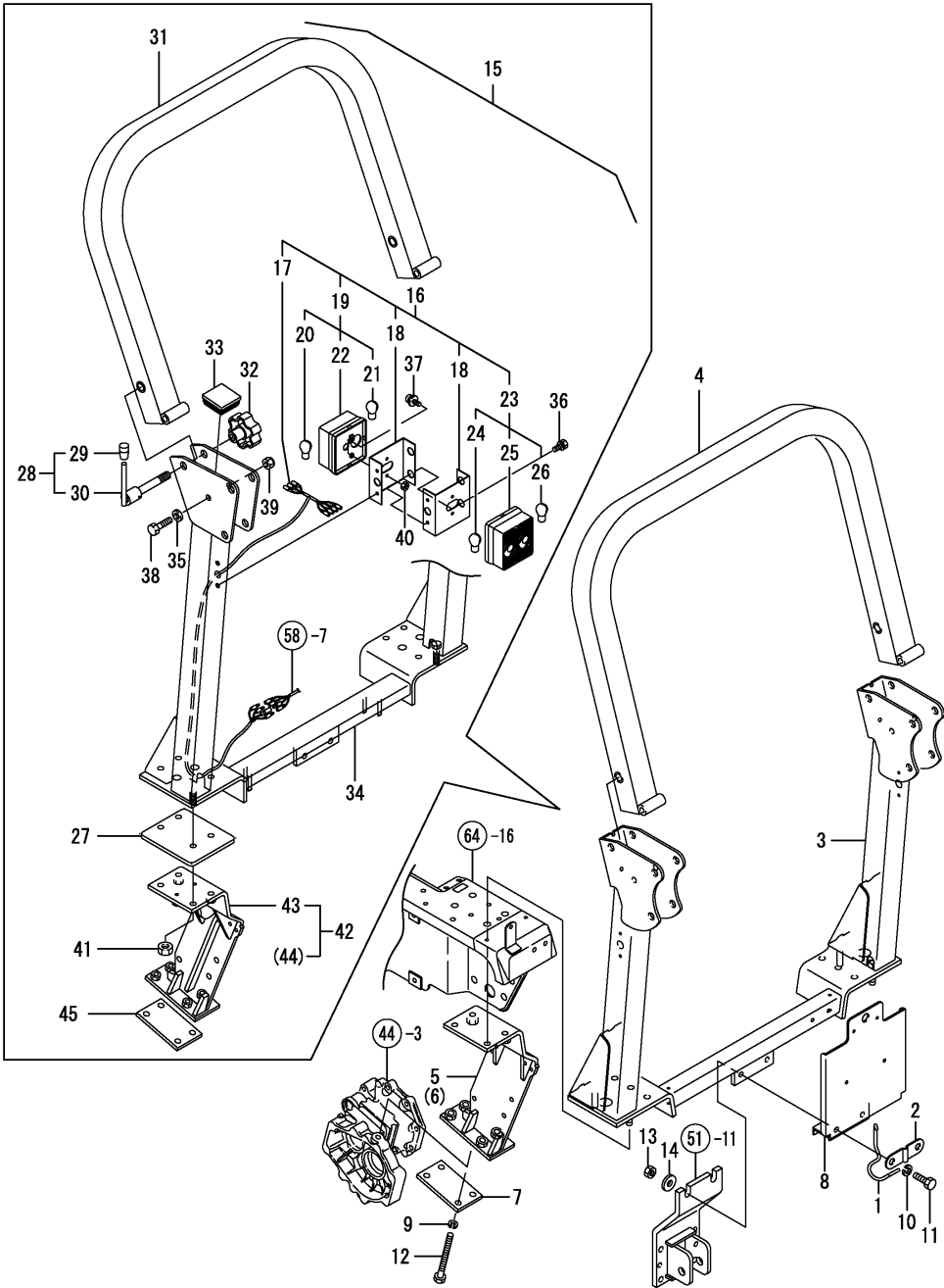
Fig.73. ROPS
