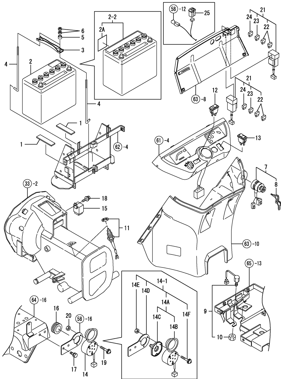
Fig.59. BATTERY & SWITCHES
