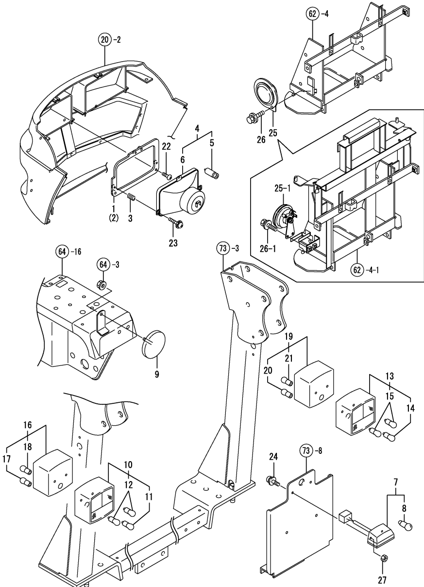
Fig.60. LAMPS & HORN
