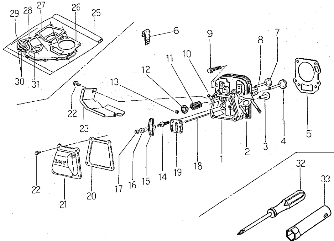
FIG.122 CYLINDER HEAD, GASKET SET, TOOLS
