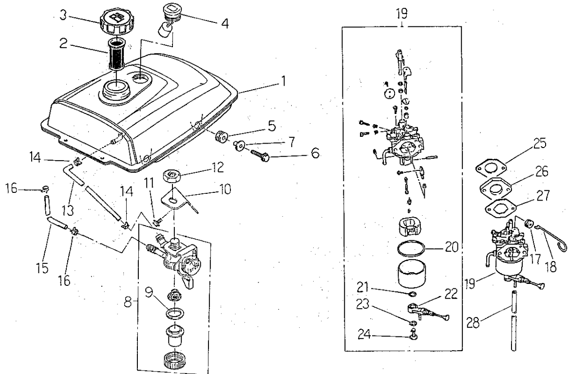
FIG. 125 FUEL TANK, CARBURETER
