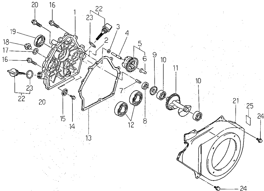
FIG.123 CRANKCASE COVER, FAN COVER
