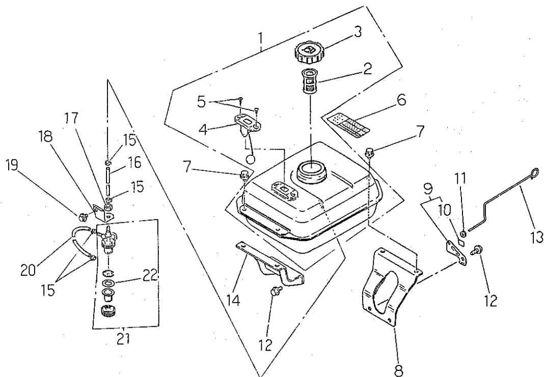
FIG.105 FUEL TANK
